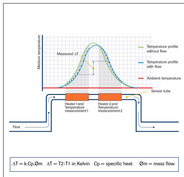
Functional scheme of thermal mass flow sensor (F-110CI)
